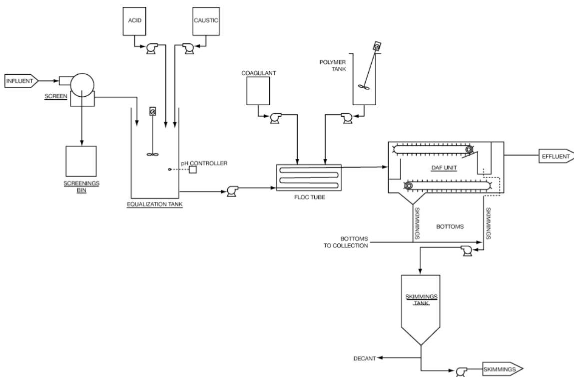
Figure 4 - Schematic Presentation of the Total Flotation System (Adapted from Ross et al., 2000)
