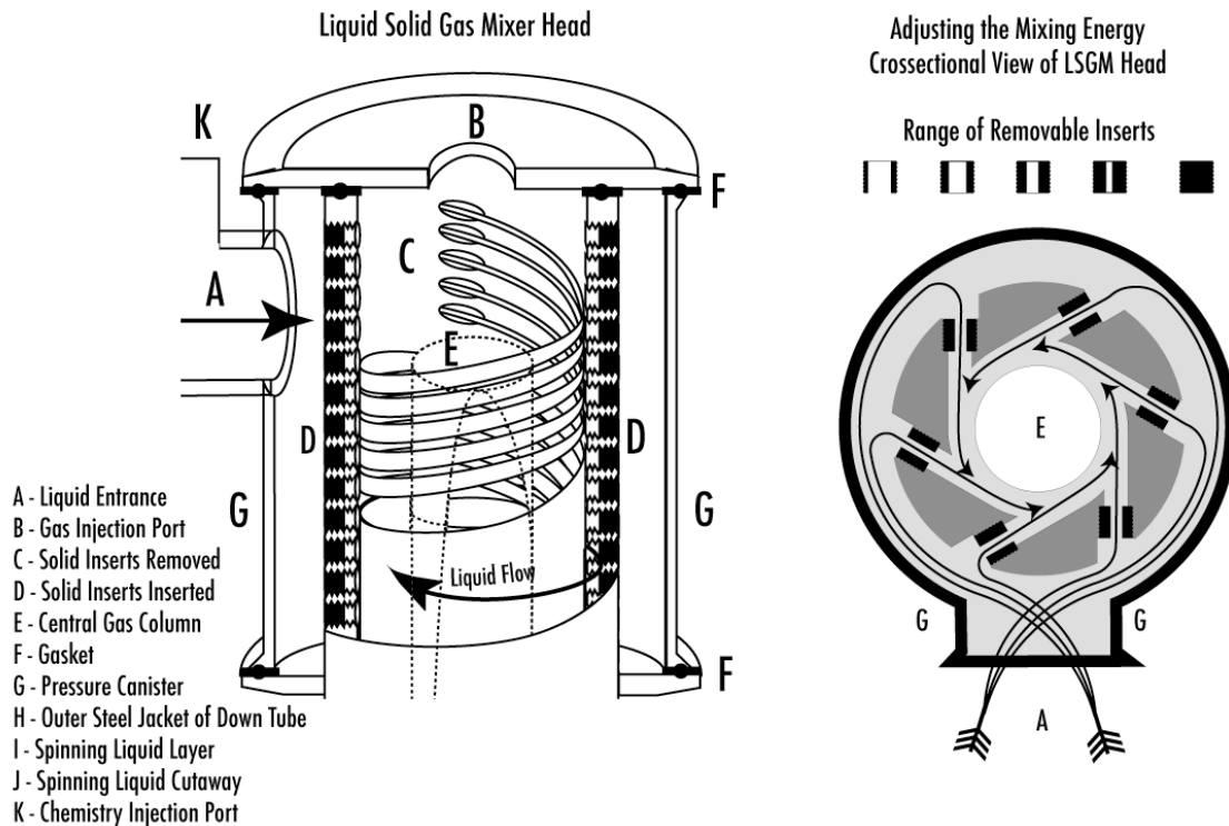
Figure 6 – Schematic Presentation of the LSGM Heads
