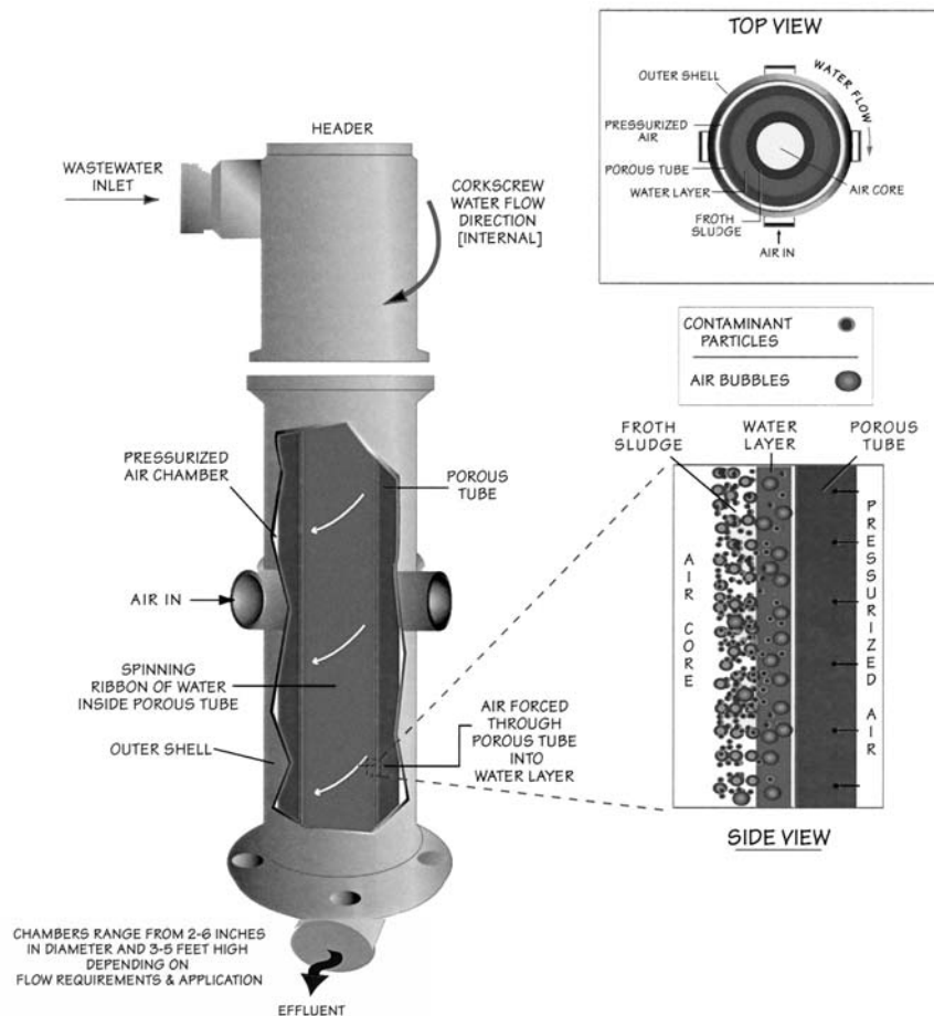
FIGURE 1. A cut-away view of a bubble chamber.
