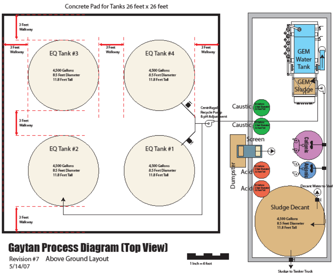
Figure 1 - Schematic Presentation of the Wastewater Treatment Plant at the Gaytan Foods
